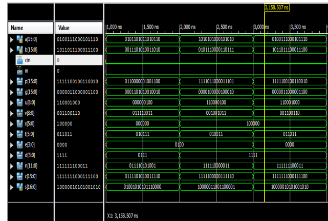
Fig.8: 16-Bit Efficient Ladner-Fischer Adder Simulation Waveform
