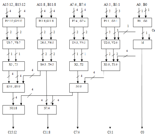
Fig.7: 16-bit Efficient Ladner-Fischer Adder
