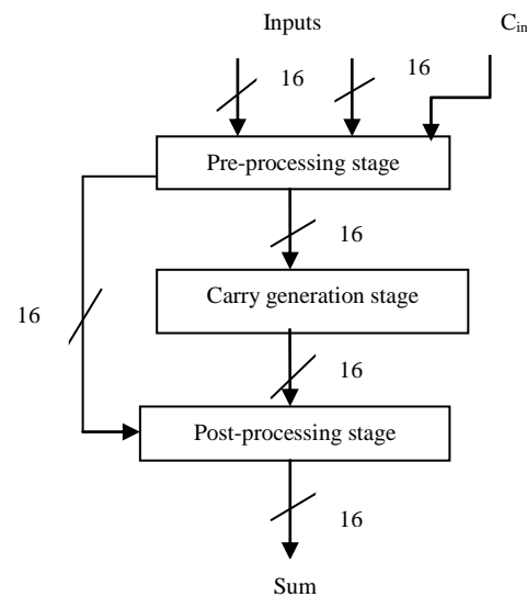
Fig.5: Block Diagram
