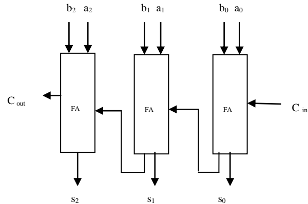
Fig.1: Three Bit Ripple Carry Adder
