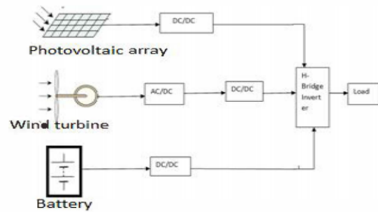
Fig I : Schematic diagram of Hybrid System
