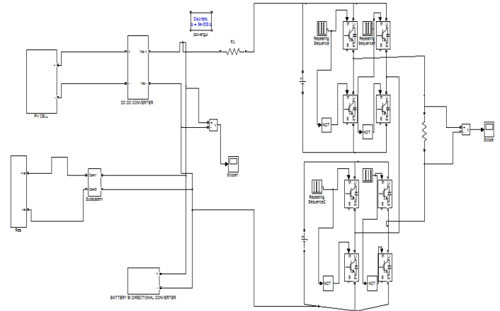
Fig.5.matlab/simulinkconventional model of without induction motor.
