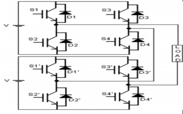
Fig 4. Five level cascaded H-bridge multilevel inverter.
