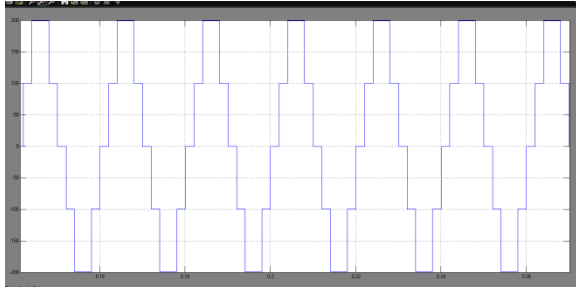
Fig 9 simulation wave form of Inverter Voltage
