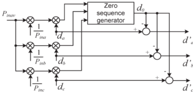
Fig. 4. Modulation compensation scheme.
