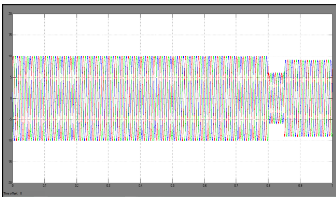
Fig 12. Three-phase grid current waveforms with modulation compensation.
