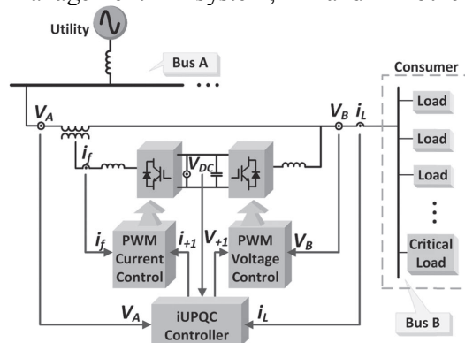
Fig 2: An modified IUPQC
