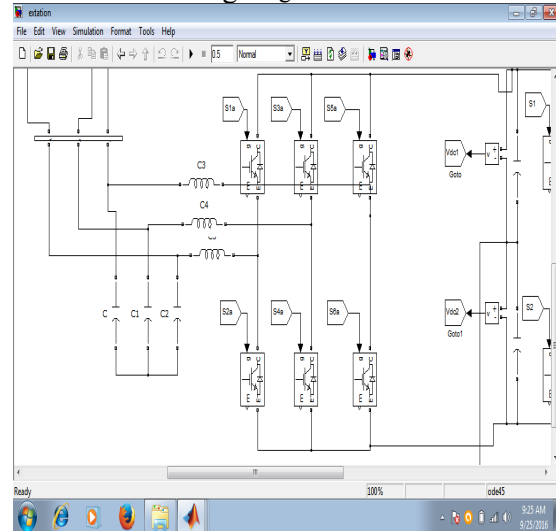
Fig 4: simulation circuit
