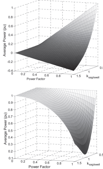
Fig 3: Apparent power of the series and shunt converters, respectively.
