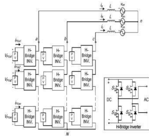
Fig. 2. Topology of the modular cascaded H-bridge multilevel inverter for grid-connected PV systems.
