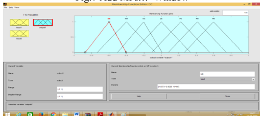
Fig8. The Updated Membership Function Editor
