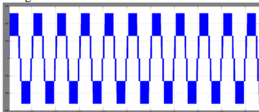
Fig15. STATCOM output voltage
