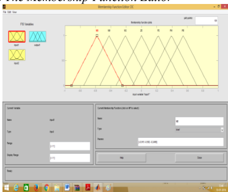
Fig6. The Membership Function Editor
