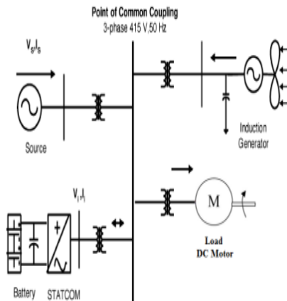
Fig.1 Grid connected system for power quality improvement
