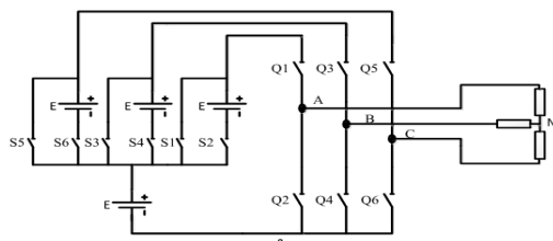
Fig2(a) Proposed three-phase MLI topology
