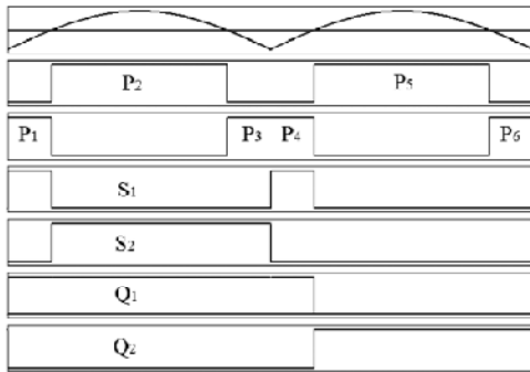
Fig 3 Switching patterns for low frequency modulation technique
