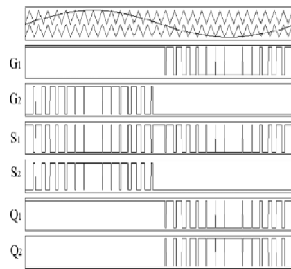
Fig. 4 Switching patterns of the proposed MLI for scheme I
