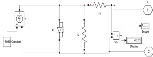
Figure 1: Single diode model of a solar cell III. PROPOSED MODULAR MLI
