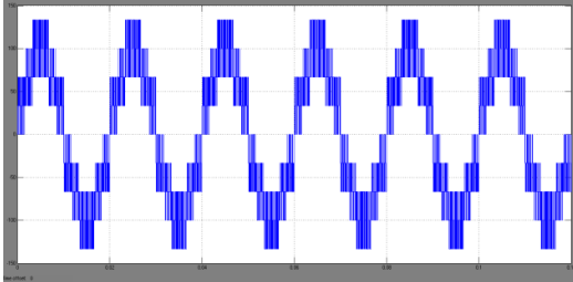
Fig. 9 phase voltages with SPWM modulation technique
