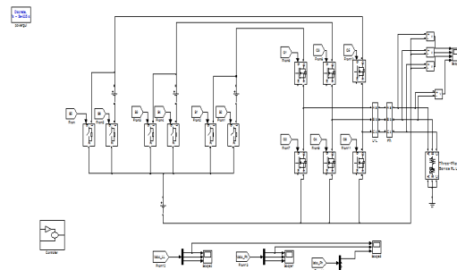
Fig. 6 SIMULINK MODEL of proposed system
