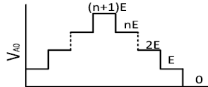
Fig 2(c) Pole voltage waveform for n-ce
