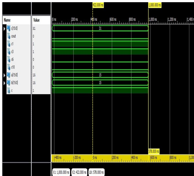
Fig1. Output Waveform of CSA using XILINX ISE
