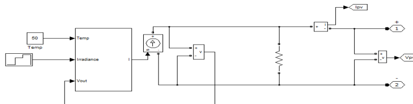
Fig 6 pv subsystem
