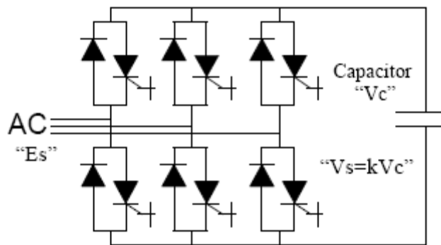
Fig.2 pulses statcom.
