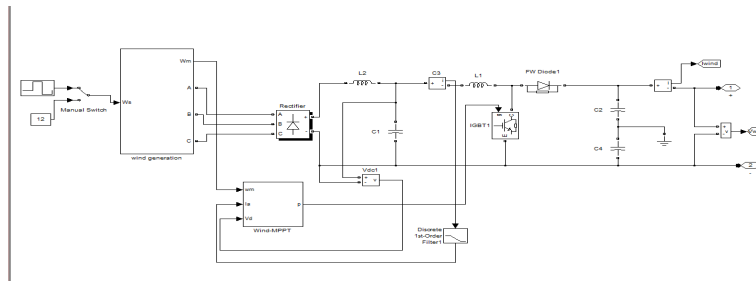
Fig7 wind subsystem
