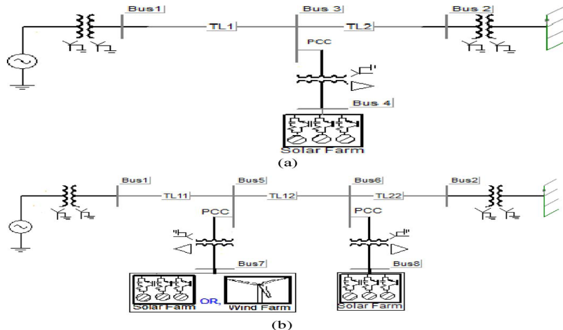
Fig3. Single-line diagram of (a) study system I with a single solar farm (DG) and (b) study system II with a solar farm (DG) and a solar/wind farm (DG).
