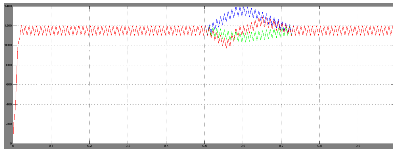
Fig 10 DC-link voltages of phase a with distributed MPPT
