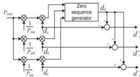
Fig. 4. Modulation Compensation Scheme
