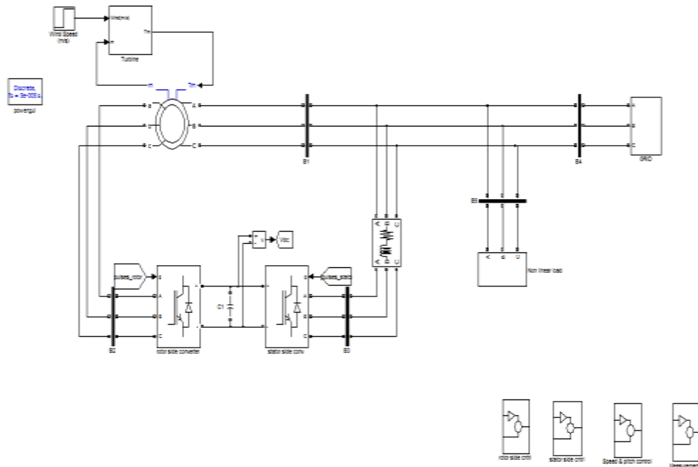
Fig 5. MATLAB/SIMULINK diagram of DFIG connected to WECS
