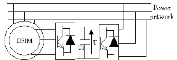
Fig. 1 Doubly-fed induction generator
