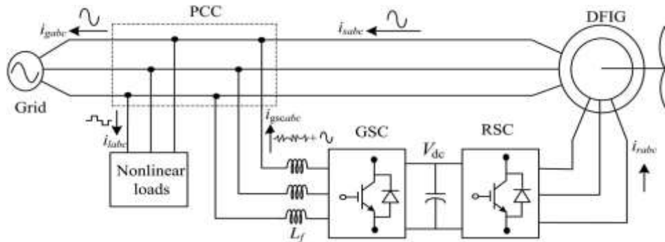
Fig.3. system configuration.
