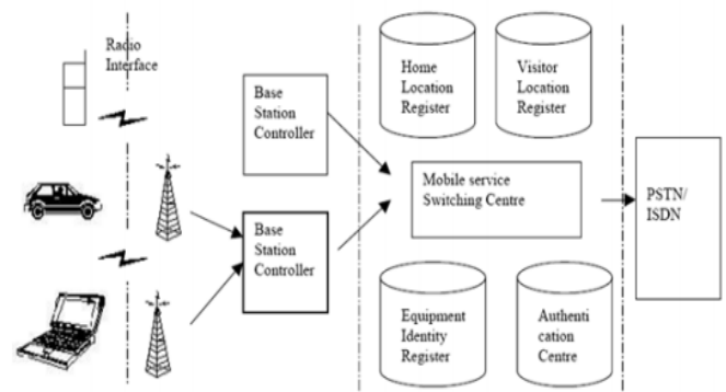
Fig 1: GSM Architecture.
