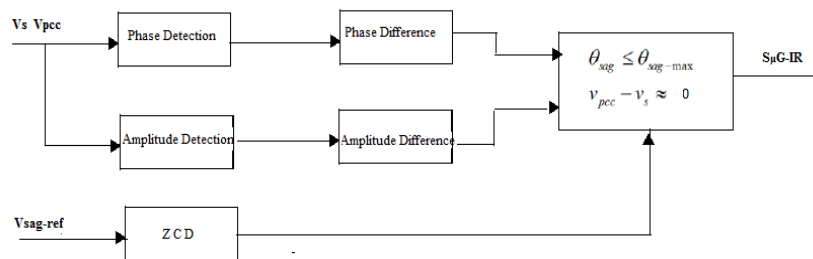
Fig 4 (a) Synchronization and Reconnection method
