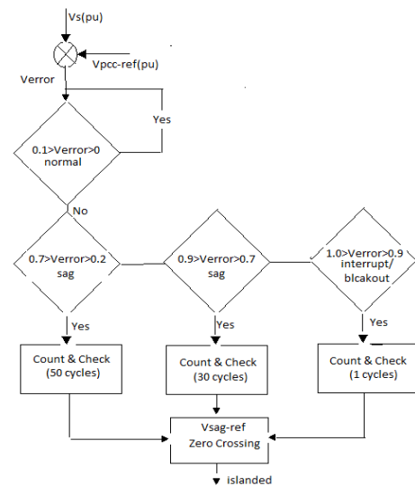
Fig 3: Algorithm for IsD method in UPQC \mu G-IR
