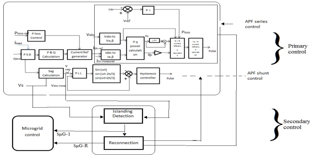
Fig 2: Block diagram of the UPQC \mu G-IR –(a) Controller (b) Control algorithm
