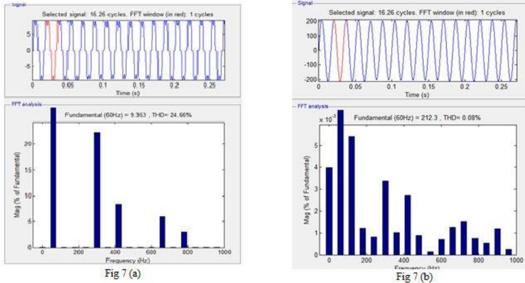
Fig 7: Total Harmonic Distortion a) Load current, b)Source current
