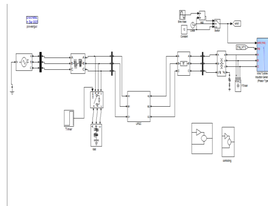
Fig :5MATLAB/SIMULINK diagram of proposed system
