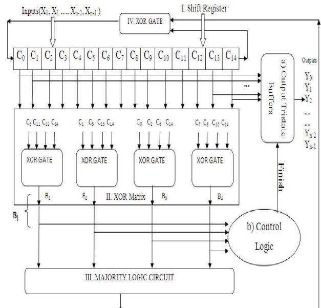
Figure 5. Schematic of the proposed MLDD for 15 bit code word. a) Control logic b) Output tristate buffers
