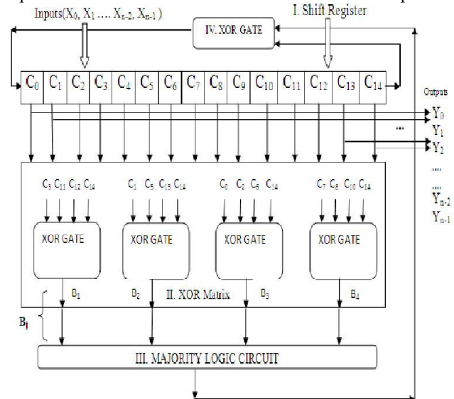
Figure 3. Serial one-step majority logic corrector for EG-LDPC code
