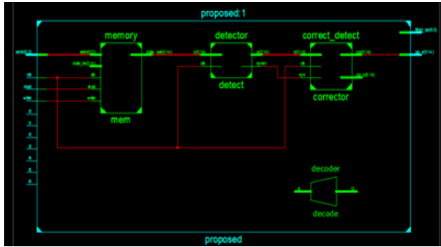
Figure 6. RTL schematic for the proposed design
