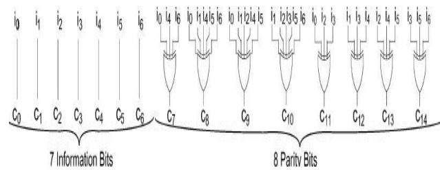
Figure 2. Structure of an encoder circuit for the EG-LDPC code
