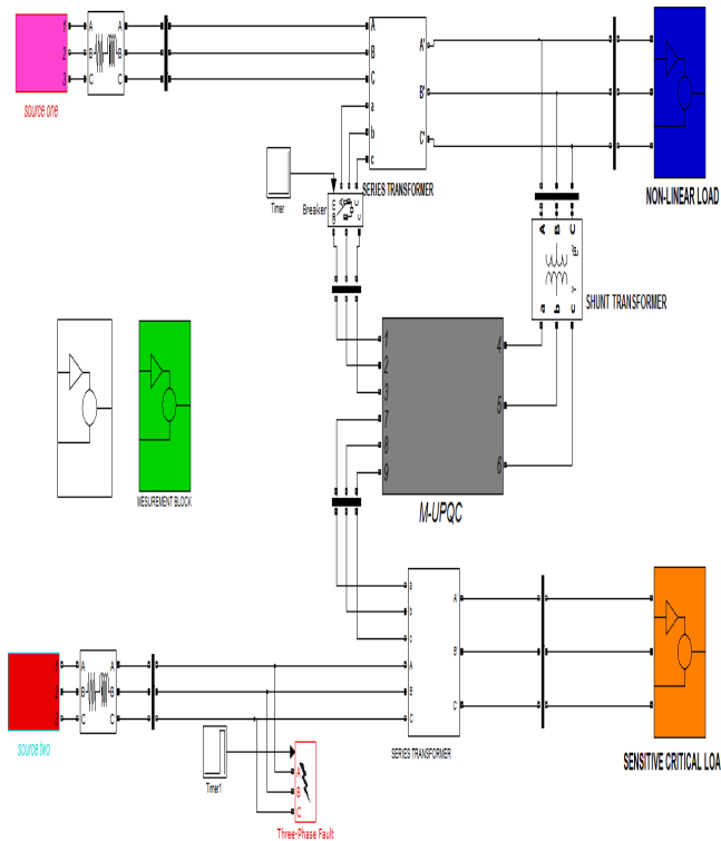
Fig.2 Typical Sim-link Block diagram MC-UPQC used in distribution system
