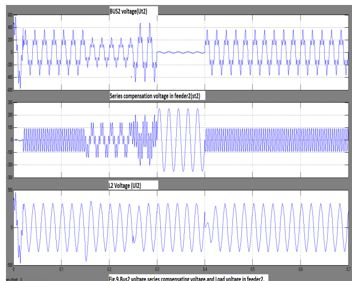
Fig.9. Bus2 voltage, series compensating voltage, and Load voltage in feeder2.
