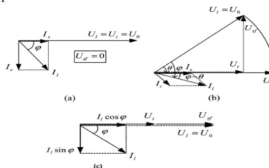
Fig.6.phasor diagram of quadrature compensation.
