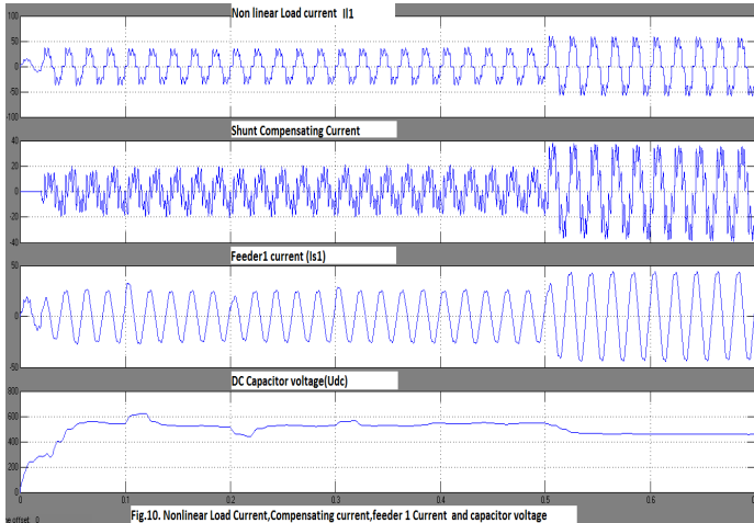
Fig.10. Nonlinear Load Current, Compensating current, feeder 1 Current and capacitor voltage
