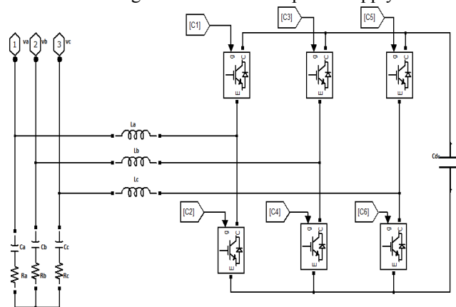
Fig.3 Schematic structure of a VSC
