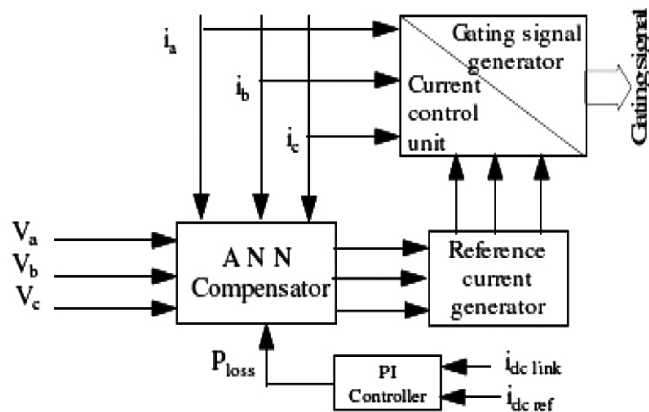
Figure.III Block diagram of ANN-based compensator
