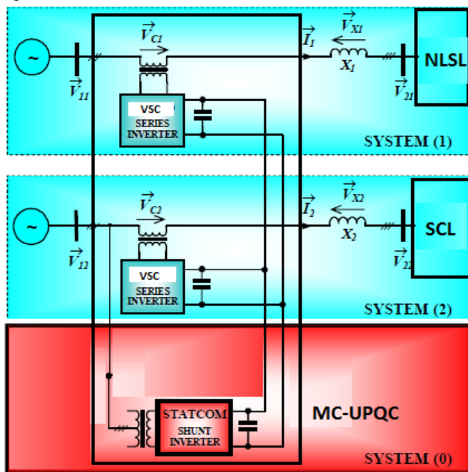
Fig.1. Block diagram of MC_UPQC with STATCOM
