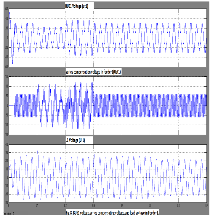
Fig.8. BUS1 voltage, series compensating voltage, and load voltage in Feeder1.
