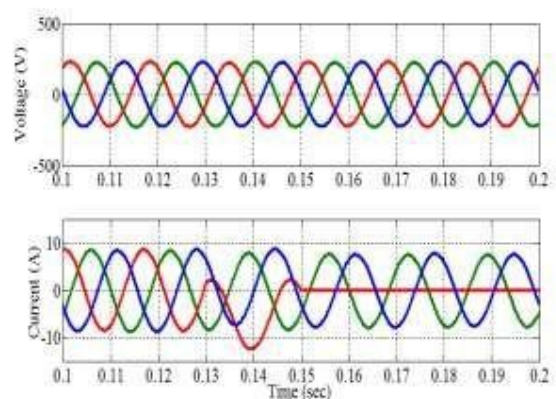
Fig.6. Simulation results of the observer based voltage control model under load step change —First: Load output voltages (V), Second: Load output currents ( I_L ).
