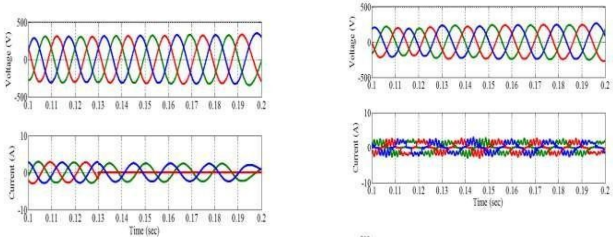
Fig. 7. Simulation results of the proposed NPC model under unbalanced load (i.e., open phase) —First: Load output voltages ( V ), Second: Load output currents ( I_L ).
