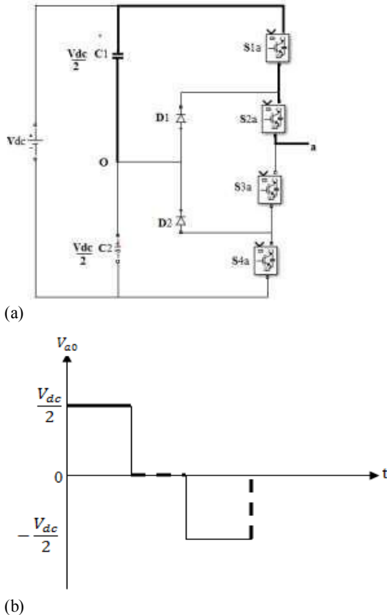
Fig.2. Operating principle of three level NPC. (a) Conducting path. (b). Corresponding output voltage.
