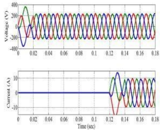
Fig.5. Simulation results of the proposed NPC model under load step change —First: Load output voltages (V), Second: Load output currents ( I_L ).
