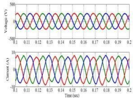
Fig. 9. Simulation results of the proposed NPC model under nonlinear load —First: Load output voltages ( V ), Second: Load output currents ( I_L ).
