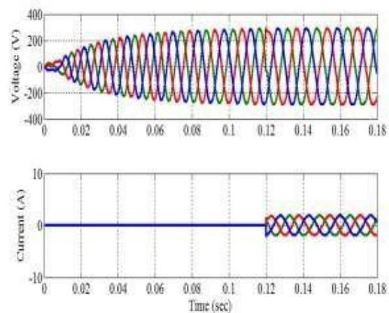
Fig.6. Simulation results of the observer based voltage control model under load step change —First: Load output voltages (V), Second: Load output currents ( I_L ).
