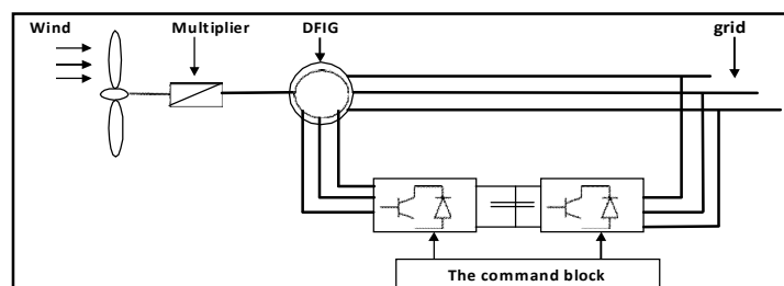
Fig 1 : DFIG in the wind energy conversion chain
