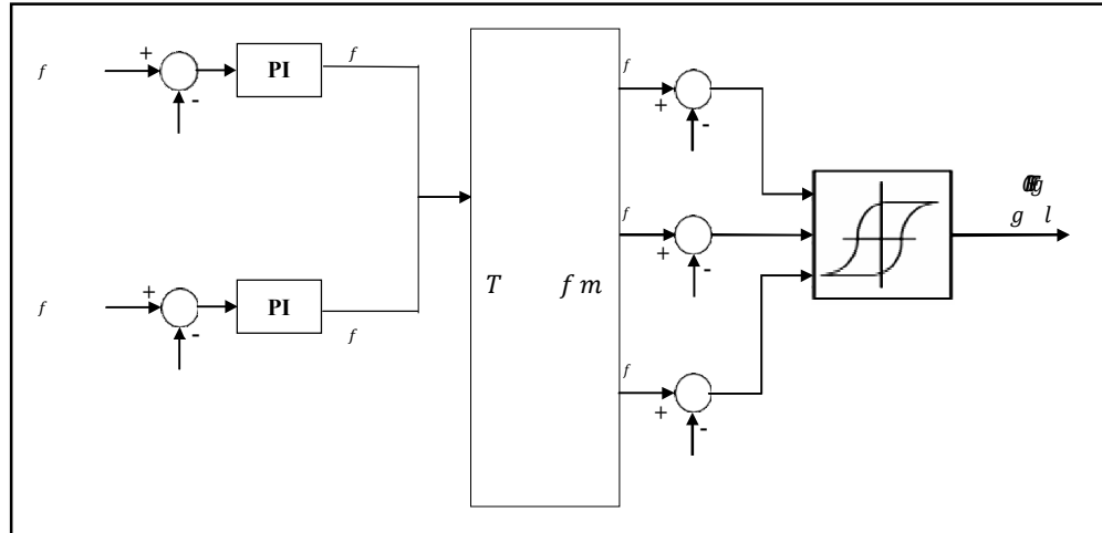
Fig 5 : Command of the DFIG [19]
