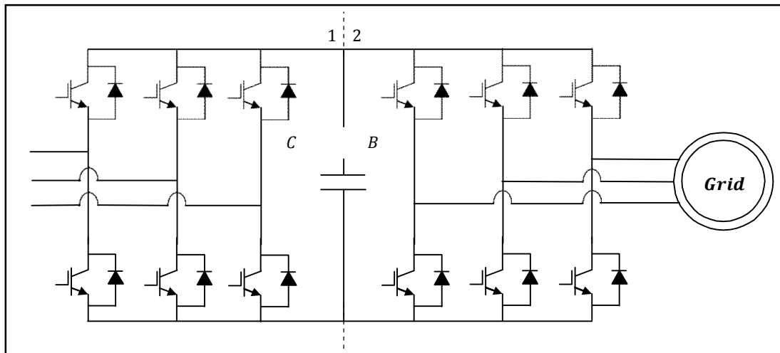
Fig 4 : Back to back converter with transistor half-bridges [22]
