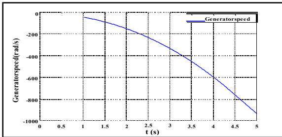
Fig 11 : Generator speed (rad/s) according to time (s)
