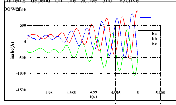
Fig 8 : Stator current isa (A), isb (A), isc (A) according to time (s)
