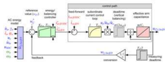
Fig.6 Effective control loop for balancing the arm energies of the MMC.
