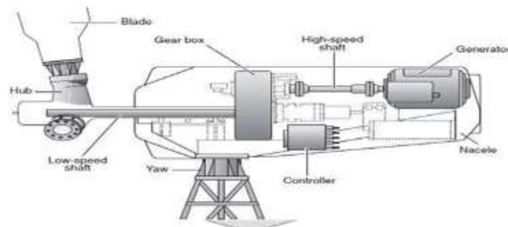
Fig-3: Horizontal axis wind mill
