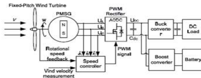
Fig-2: Topology of non grid connected wind energy conversion system
