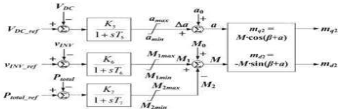
Fig-7: control block diagram of the modulation indices of grid VSI
