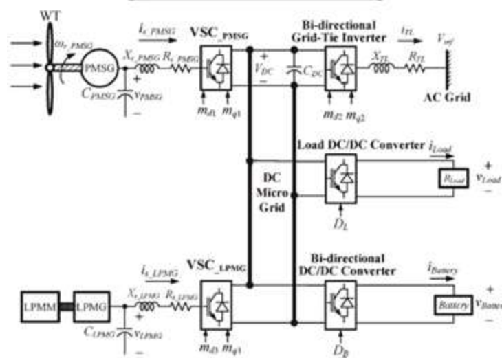
Fig-1: Configuration of the studied integrated wind and wave power generation system connected to a power grid through the proposed dc microgrid.
