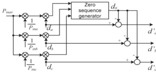
Fig. 4. Modulation compensation scheme.
