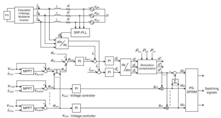
Fig. 3. Control scheme for three-phase modular cascaded H-bridge multilevel PV inverter.
