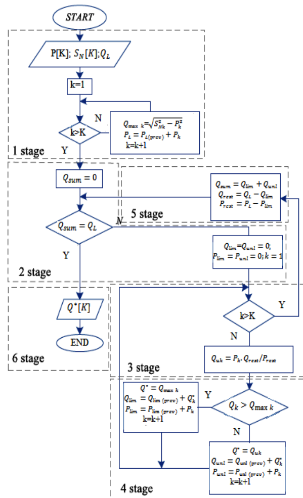
Fig. 5: Block diagram of developed reactive power sharing algorithm.
