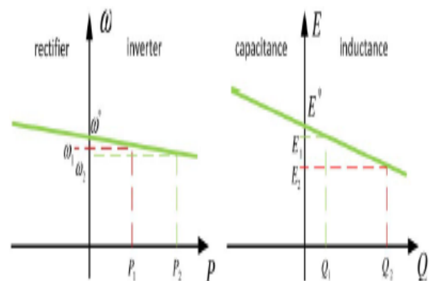
Fig. 2: P- \omega and Q-E droop characteristics.
