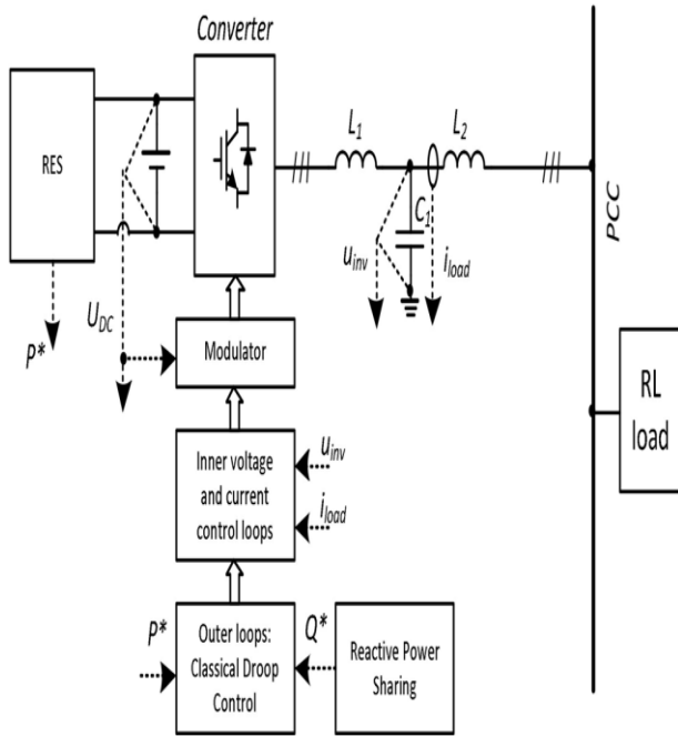
Fig. 3: Block scheme of control structure for one of the converters in islanded MG.
