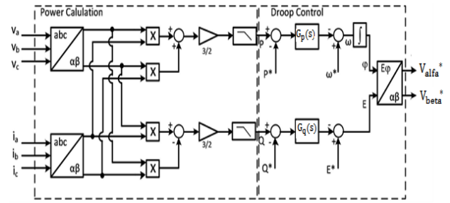
Fig. 4: Block scheme of classical droop control.
