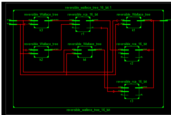
Fig 12 RTL of 16- bit Multiplier using Reversible logic
