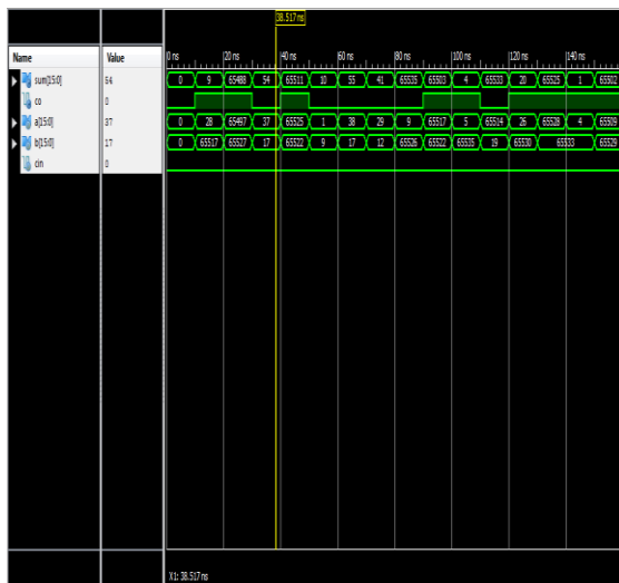
Fig 9 Output wave form of 16- bit adder using Reversible logic
