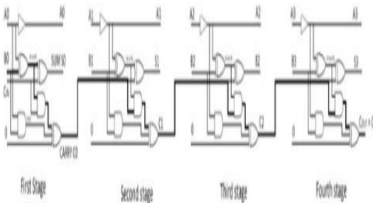
Fig1.Critical Path of 4-bit reversible adder
