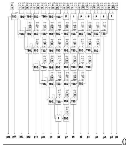
Fig4. 2.12 8X8 reversible Wallace tree Multiplier
