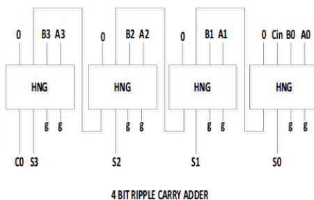
Fig3:4 Bit Ripple Carry Adder 4.WALLACE TREE MULTIPLIER
