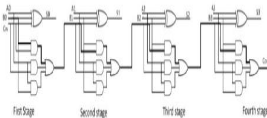
Fig2. Critical Path of 4 bit irreversible adder
