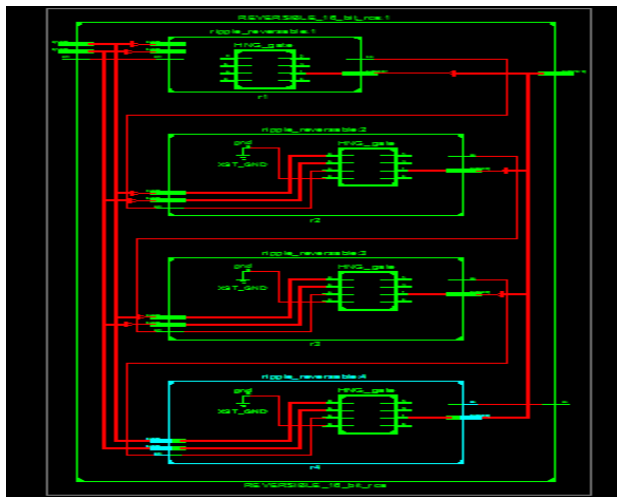
Fig 8 RTL of 16- bit adder using Reversible logic
