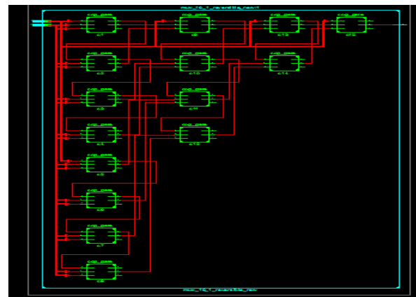
Fig 10 RTL of 16- bit MUX using Reversible logic
