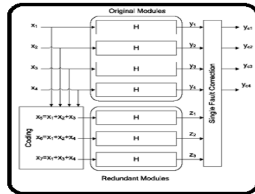
Fig.1. Framework of Filters & Hamming code.
