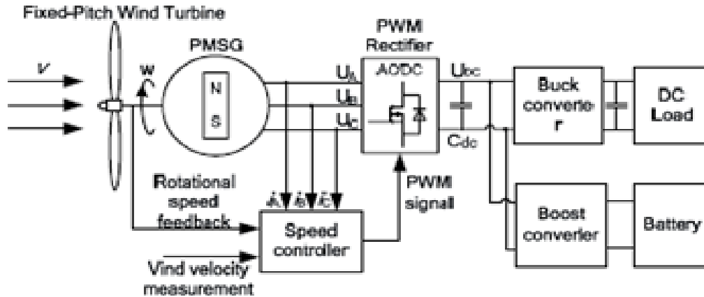
Fig-2: Topology of non grid connected wind energy conversion system
