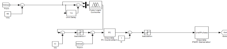
Fig 9. Load side controller
