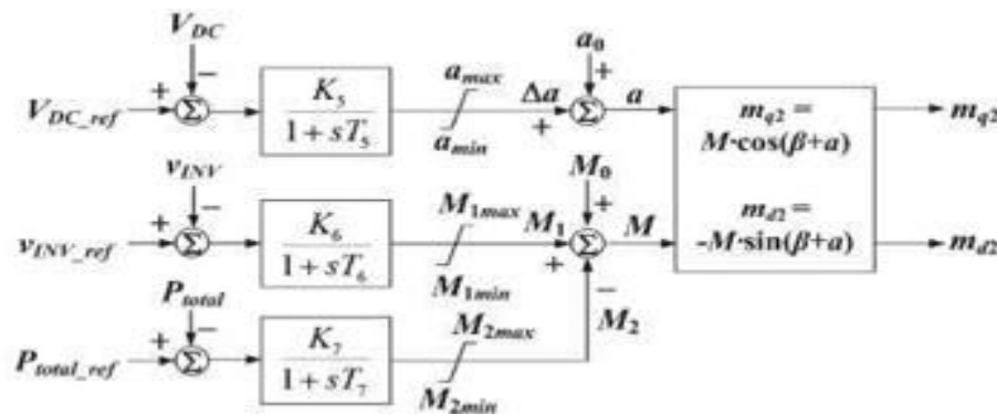
Fig-7: control block diagram of the modulation indices of grid VSI
