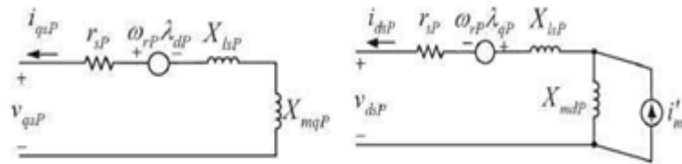
Fig-4: q-d axis equivalent circuit model of the studied wind PMSG
