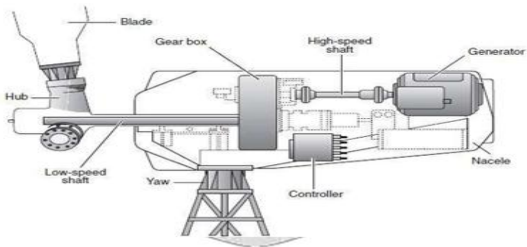
Fig-3: Horizontal axis wind mill
