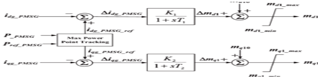
Fig-6: Control block diagram of the modulation indices of the VSC of the studied PMSG.
