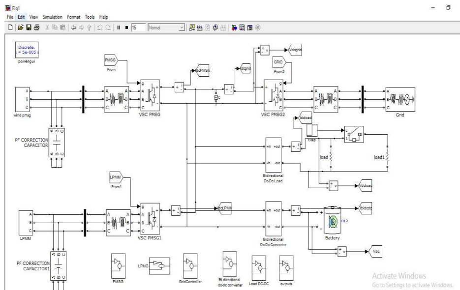
Fig 8. MATLAB/SIMULATION diagram of proposed wind and wave system
