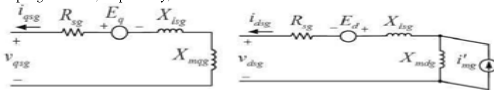
Fig-5: q - d -axis equivalent circuit model of the studied LPMG.
