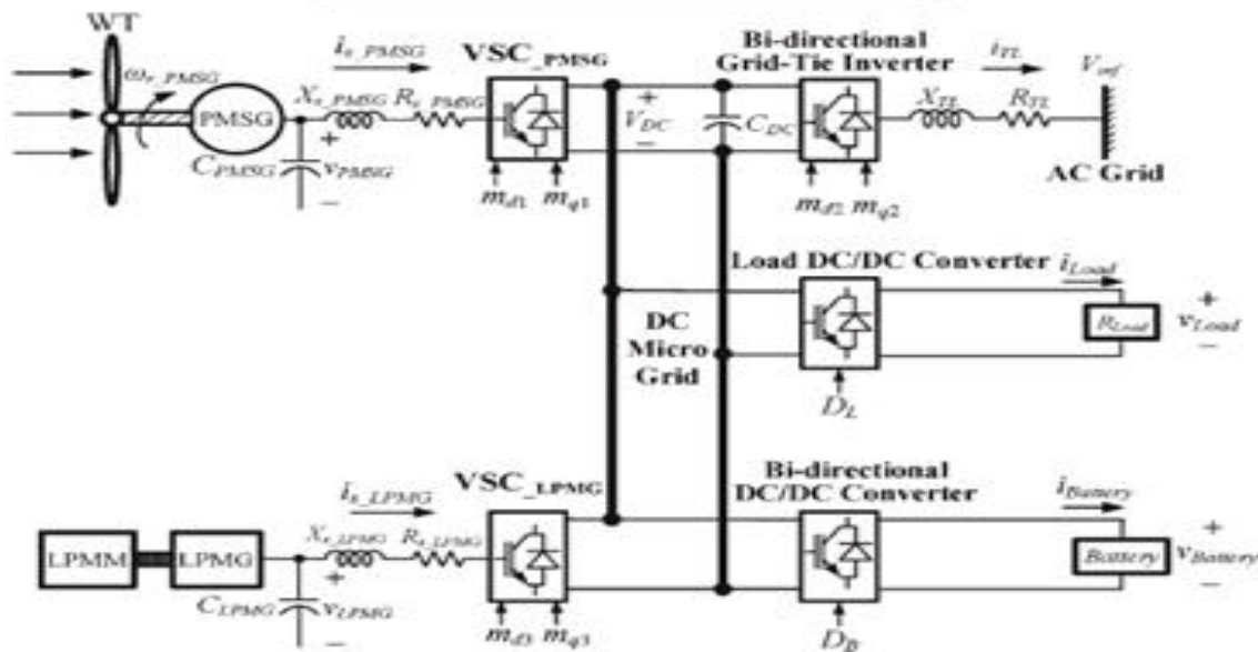
Fig-1: Configuration of the studied integrated wind and wave power generation system connected to a power grid through the proposed dc microgrid.
