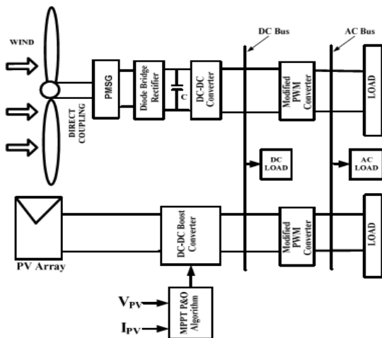
Fig.1. Block diagram of Implemented Hybrid System with Modified PWM converter Topology.
