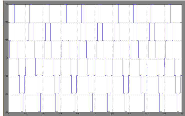
Fig 5 simulation wave form of conventional method seven level inverter
