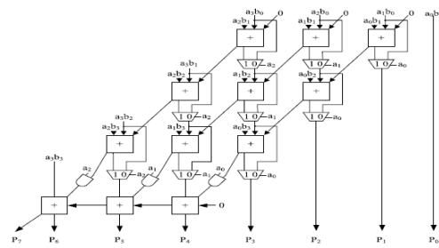
Fig 1 column-bypassing multiplier.
