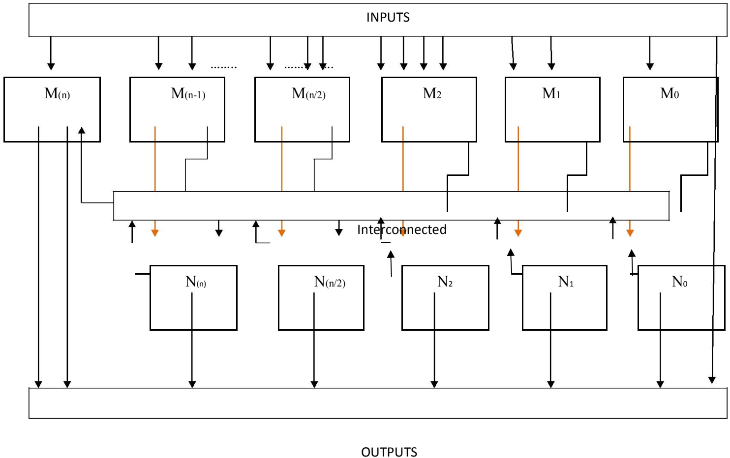
Fig. 2 4 x 4 HIGH PERFORMANCE TRIGIC LOGIC MULTIPLIER
