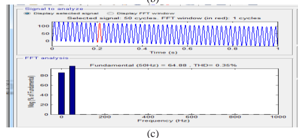
Fig 9 (a) nine level Output voltage of inverter (b) In phase waveform of grid voltage and grid current (c) Harmonic Analysis of Grid Current
