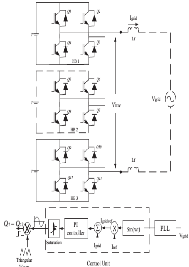
Fig. 3. Circuit diagram of Cascaded Seven level Inverter for single phase Grid Connected System
