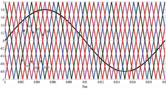
Fig. 2. Phase shift PWM for seven-level inverter
