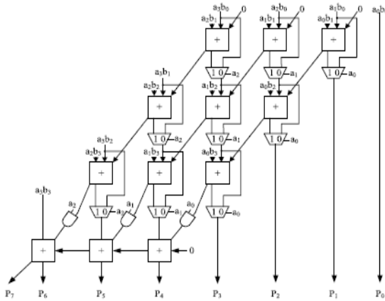
Fig. 2. 4 × 4 column-bypassing multiplier.
