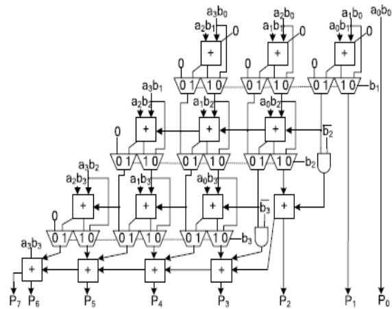
Fig. 3. 4 × 4 row-bypassing multiplier.
