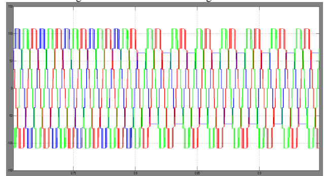
Fig 16 Simulation waveform of Inverter voltage
