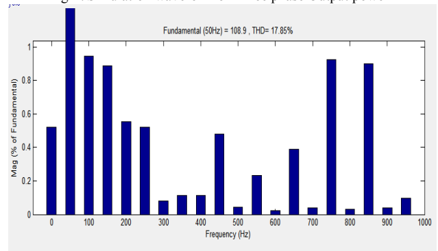
Fig 18 Simulation waveform of Harmonic analysis
