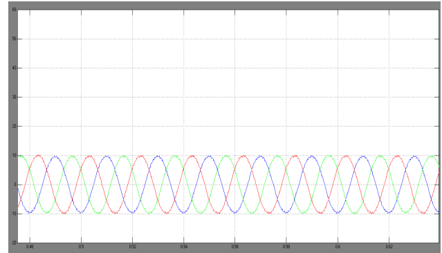
Fig 15 Simulation waveform of grid current
