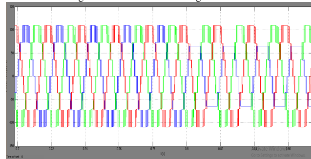
Fig 9 Simulation waveform of output MLI voltage
