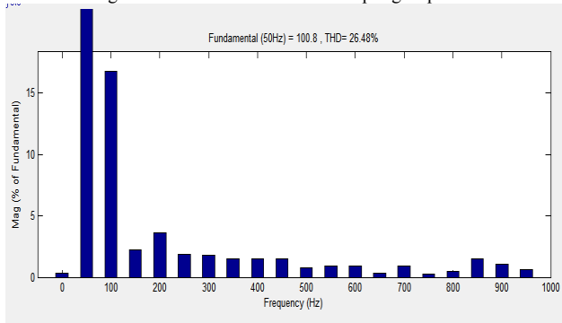
Fig 12 Simulation waveform of harmonic analysis
