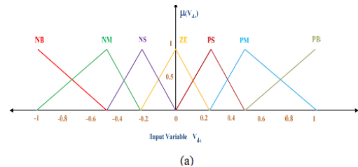
Fig 4 Conventional fuzzy controller
