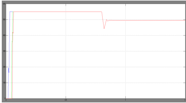
Fig 11 Simulation waveform of output grid power
