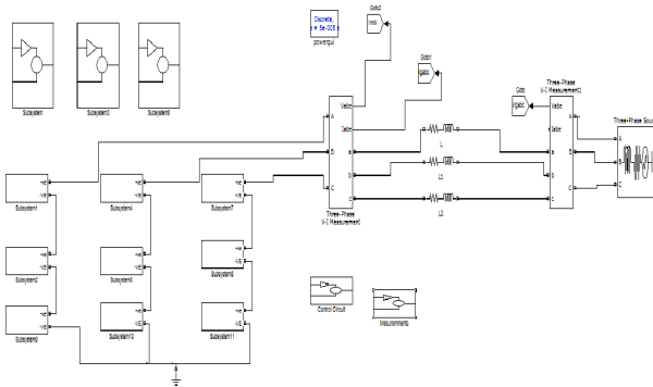
Fig 6 Simulation model of modular cascaded distributed MPPT control based grid connected system
