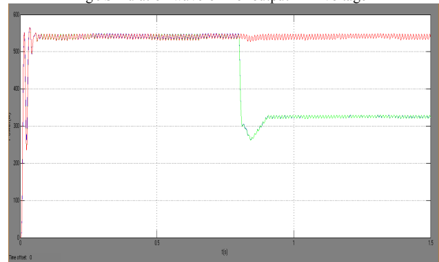
Fig 10 Simulation waveform of Power extracted from PV panel
