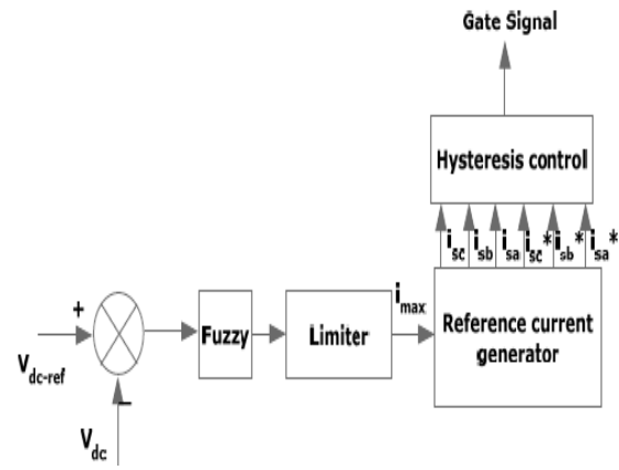
Fig 4 Conventional fuzzy controller
