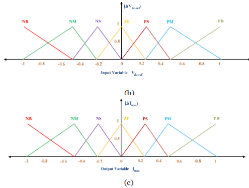
Fig 5(a) Input Vdc normalized membership function; (b) Input Vdc-ref Normalized Membership Function; (c) Output Imax Normalized Membership Function
