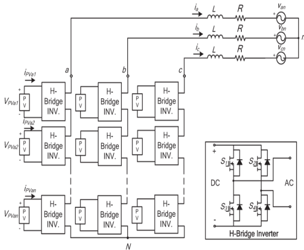
Fig. 1. Topology of the modular cascaded H-bridge multilevel inverter for grid-connected PV systems.
