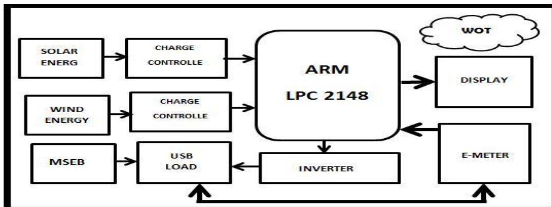
Fig 3: Block Diagram of WoT and energy management system.
