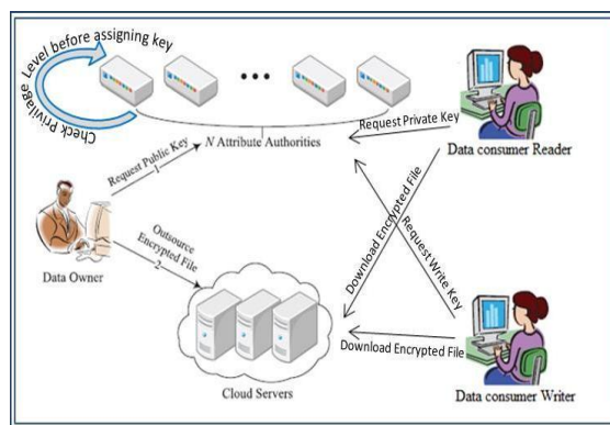
Fig 1.1: architecture of system
