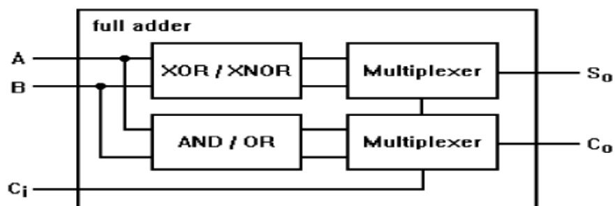
Figure 1: Alternative logic scheme for designing full-adder cells.
