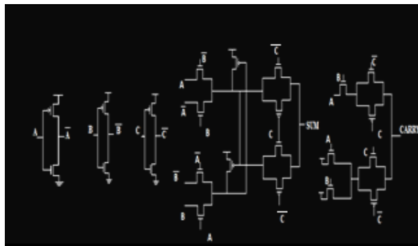
Figure 2: Full-adder designed with the Proposed Logic structure and a Pass Transistor Logic Style
