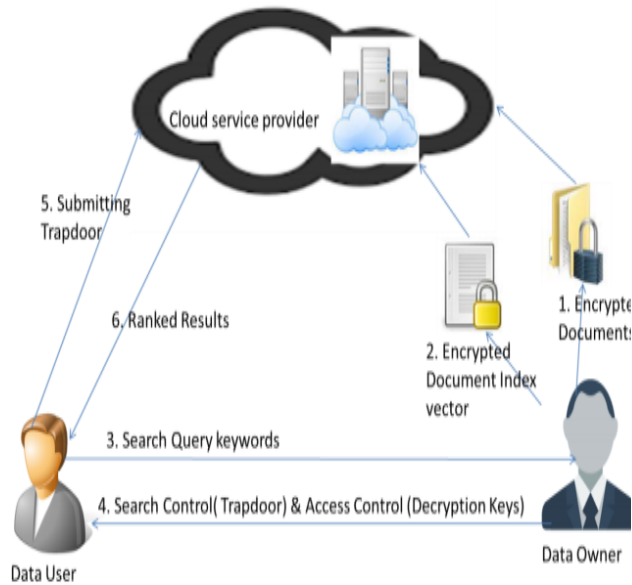
Fig No 2 System Model
