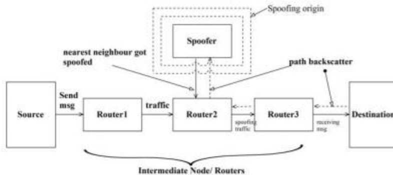
Fig. 1. Architecture of proposed work
