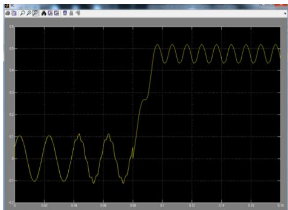
Fig 5: Minimized dc component of Grid current waveforms by single integral
