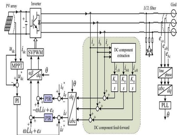
Fig 2: DC component minimization strategy based on dc component feed-forward and PIR controllers.
