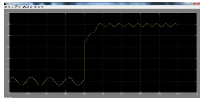
Fig 7: Minimized dc component of Grid current waveforms by single integral with fuzzy controller
