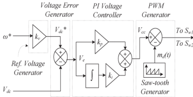
Fig. 5. PI Control of the PFC BL-CSC converter feeding BLDC motor drive.
