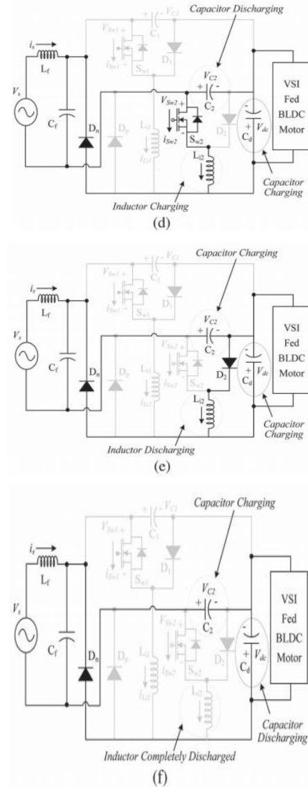
Fig. 4. Different modes of operation of the proposed BL-CSC converter. (a) Mode I-A. (b) Mode I-B. (c) Mode I-C. (d) Mode II-A. (e) Mode II-B. (f) Mode II-C.
