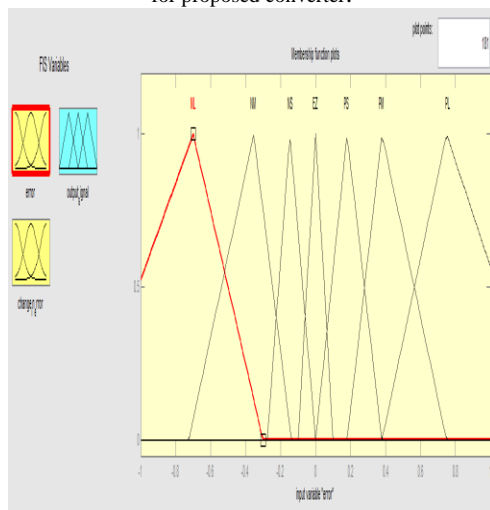
Fig.9. Membership functions for error.
