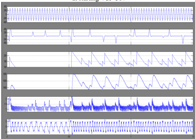
Fig 14 simulation wave form of conventional converter of source voltage, source current, dc link voltage, speed, torque and stator currents during speed control and change in dc link voltage.
