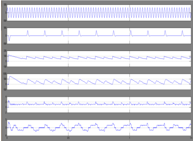
Fig 13 simulation wave form of conventional converter of source voltage, source current, dc link voltage, speed, torque and stator currents at starting V_{dc}=50v
