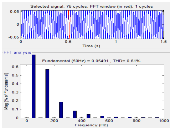
Fig.18.THD for Fuzzy logic controller Current.
