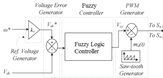
Fig. 7. Fuzzy logicControl of the PFC BL-CSC converter feeding BLDC Motor Drive.
