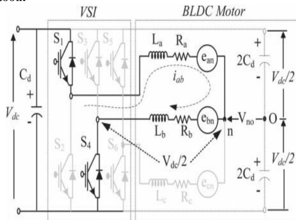
Fig. 6. Three-phase VSI feeding a BLDC motor.
