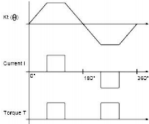
Fig.2 Waveform of current and torque.
