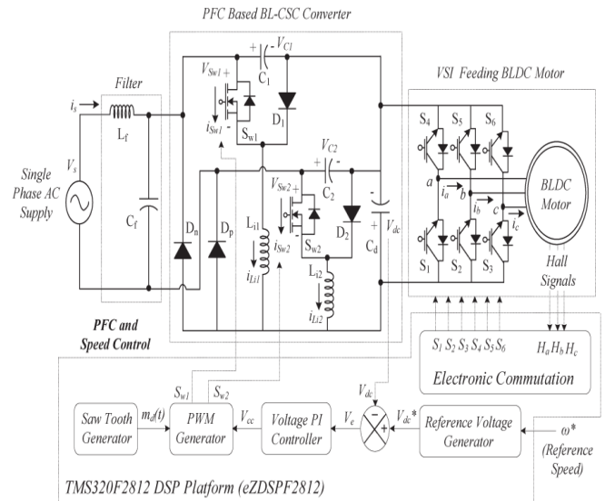
Fig.3. Proposed BL-CSC converter-fed BLDC motor drive.
