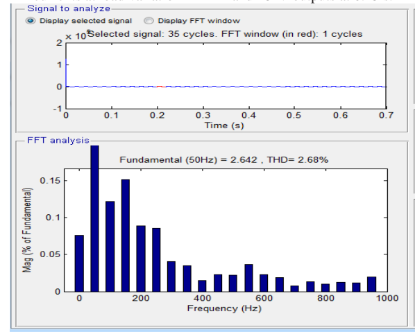
Fig 9 THD analysis of the system
