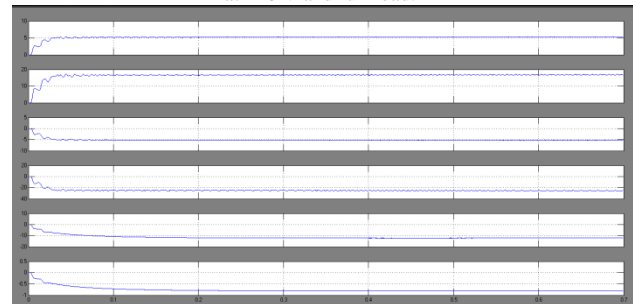
Fig 8 simulation wave form of Input voltage, current, bridgeless buck boost converter output voltage, half-bridge VSI output voltages, and currents at load variation in +12- and +5-V outputs at 0.25 s.
