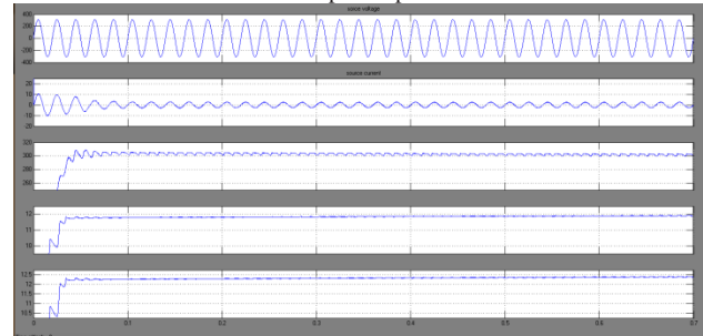
Fig 7 simulation wave form of Input voltage, current, buck-boost converter output voltage, half bridge VSI output voltages, and currents at 220 V and full load.
