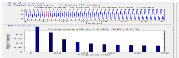
Fig 13 THD analysis of current with fuzzy logic controller
