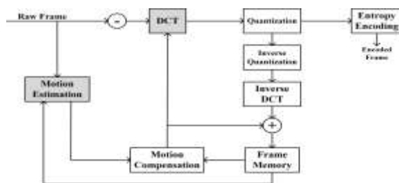
FIG. 2 EXISTED SYSTEM
