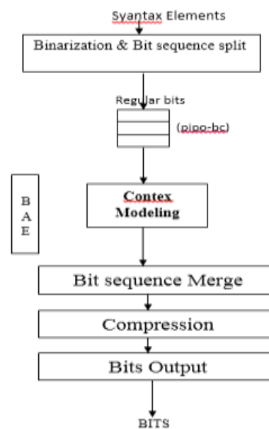
FIG. 3 PROPOSED SYSTEM
