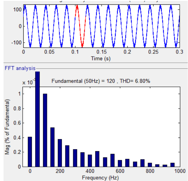
Fig.15.T total harmonic distortion for UPQC compensated system, Base THD =6.80%.
