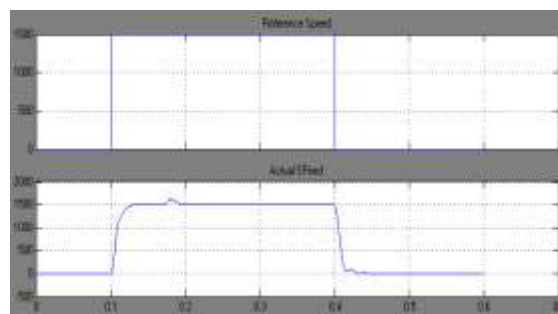
Fig: 9. Reference speed and actual speed in rpm.
