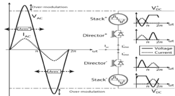
Fig. 3. Idealized voltage and current waveforms over one cycle in a phase converter of the AAC, showing the working period of each arm.
