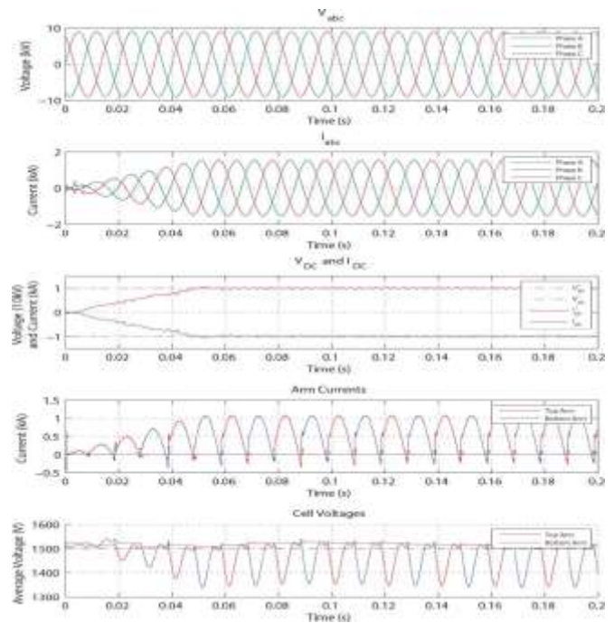
Fig. 5. Simulation results of a 20-MW AAC model running in rectifier mode under normal conditions.
