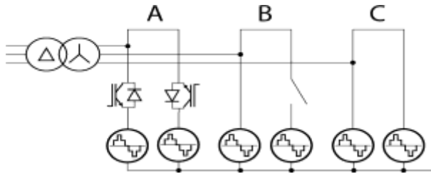
Fig. 4. STATCOM modes of the AAC during a dc-side fault: alternate arms (mode A), single working arm (mode B), and dual working arms (mode C).
