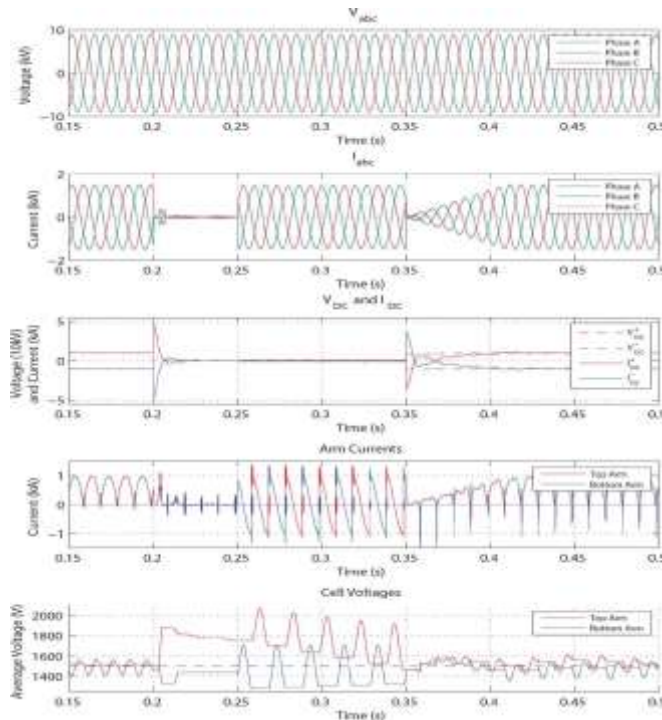
Fig. 8. Simulation results of a 20-MW AAC model running in rectifier mode when a dc-side fault occurs between 0.20 and 0.35 s.
