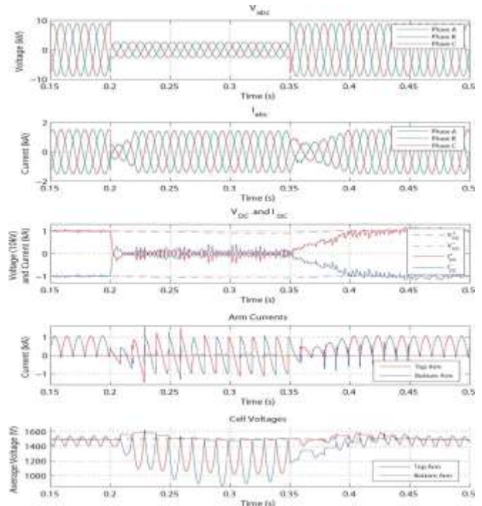
Fig. 7. Simulation results of a 20-MW AAC model running in rectifier mode when an ac-side fault occurs between 0.20 and 0.35 s.
