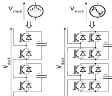
Fig. 1. Electrical schematic of half-bridge cells (left) and H-bridge cells (right).
