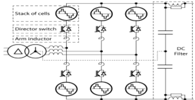
Fig. 2. Schematic of the alternate arm converter, with the optional middle-point connection shown in a dashed line.
