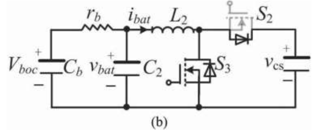
Fig.8. Equivalent circuit of the battery with (a) the buck converter in charge mode and (b) the boost converter in discharge mode.
