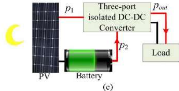
Fig.5. Three working scenarios of the converter (the arrows show the directions of energy flow). (a) Scenario 1 ( p_1 > p_{out} ): PV works in MPPT mode and the battery works in charge mode to absorb the surplus solar energy. (b) Scenario 2 ( p_1 < p_{out} ): PV works in MPPT mode and battery works in discharge mode to provide the deficient energy. (c) Scenario 3 ( p_1 = 0 ): there is no solar energy available and battery is discharged to supply load.
