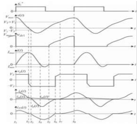
Fig.3. Steady-state waveforms of the proposed converter.
