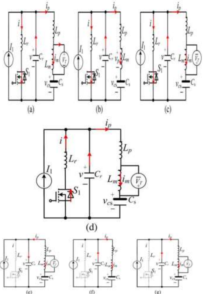
Fig. 4. Equivalent circuits for different operating modes. (a) Mode 1: S1 is on, i > 0 , and v_p = V_T . (b) Mode 2: S1 is on, i > 0 , and i_p = i_m . (c) Mode 3: S1 is on, i > 0 , and v_p = -V_T . (d) Mode 4: S1 is being turned off, i < 0 , and v_p = -V_T . (e) Mode 5: S1 is off, i = 0 , v_p = -V_T . (f) Mode 6: S1 is off, i = 0 , and i_p = i_m . (g) Mode 7: S1 is off, i = 0 , and v_p = V_T .
