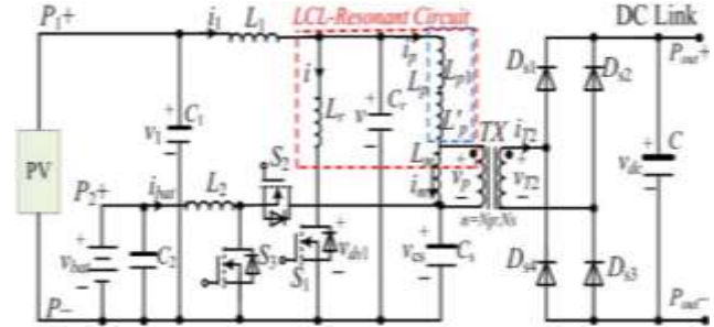
Fig. 1. Proposed isolated three-port bidirectional dc-dc converter for a PV and battery system.
