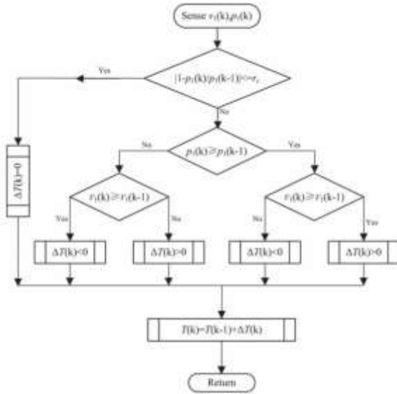
Fig.7. Flowchart of the MPPT algorithm.
