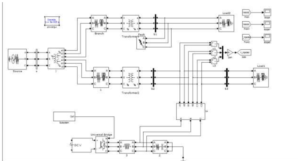
Fig. MATLAB/SIMULINK diagram of proposed system single phase sag
