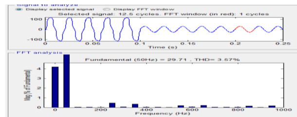
Fig 10 Simulation waveform for reverse reactive power
