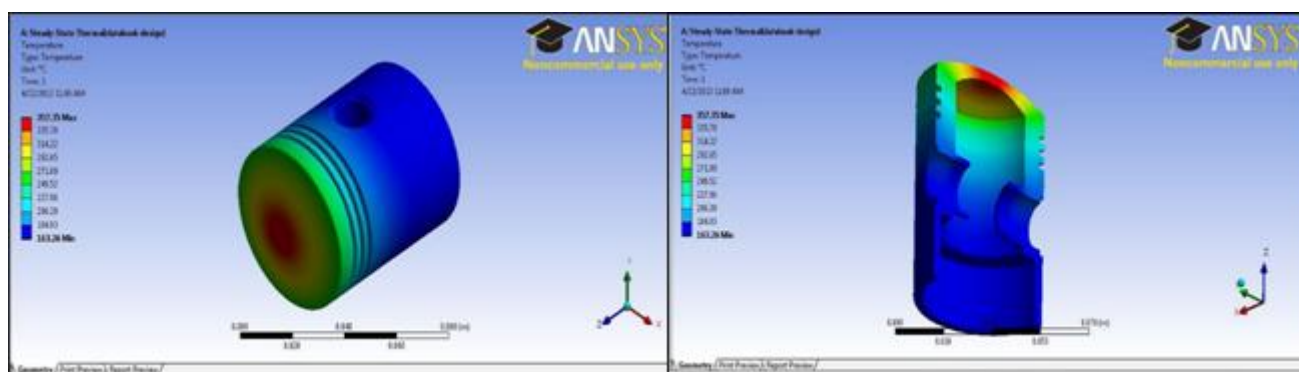
Fig 3(c): Temperature profile of the piston
