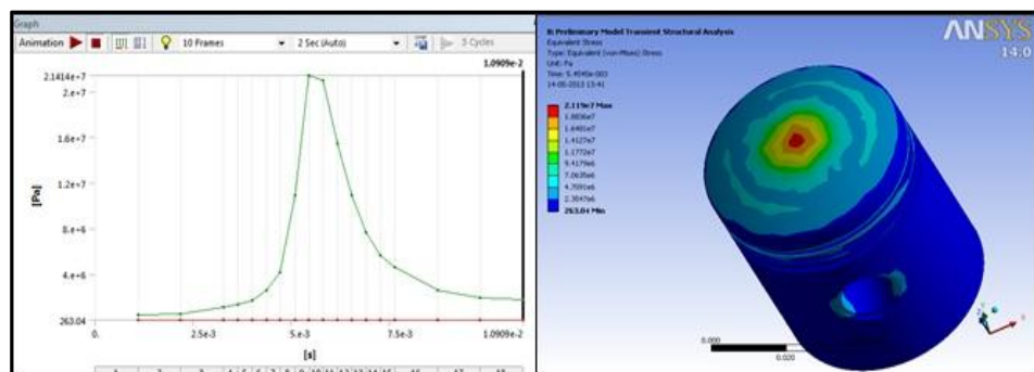
Fig 3(a): Von Mises Stress distribution
