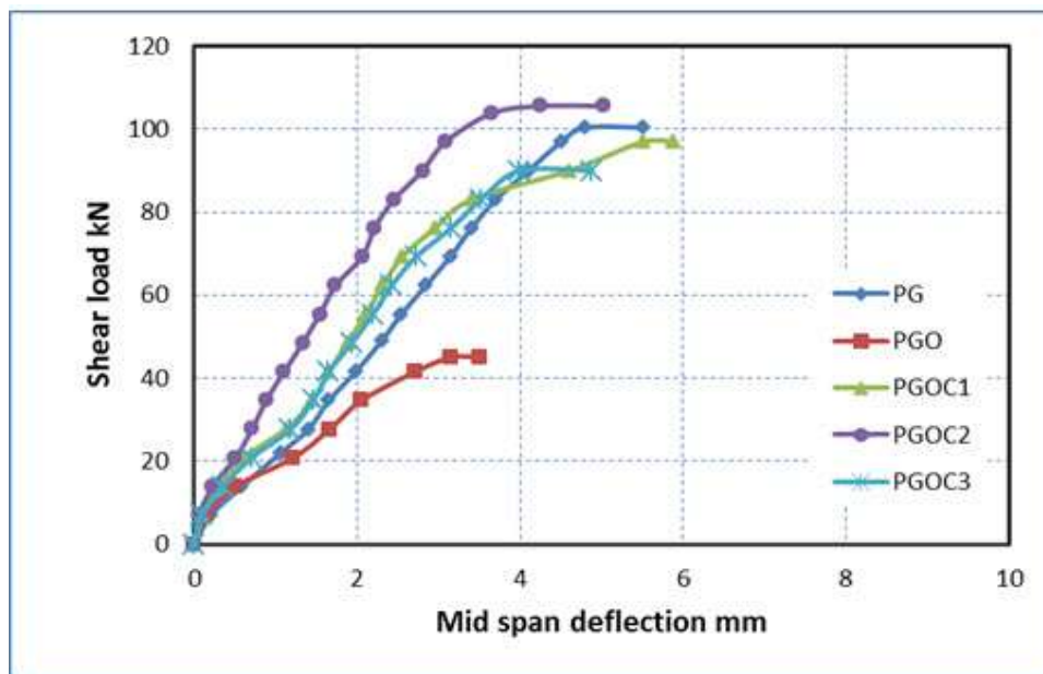
Figure(5):Load-deflection curves for PG,PGO,PGOC1,PGOC2 and PGOC3
