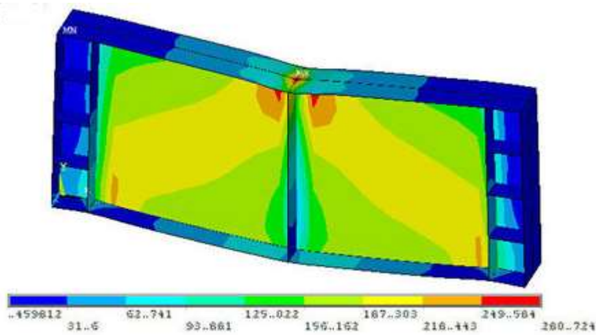
Figure (8): Von Mises stress distribution of plate girder (PG) at failure
