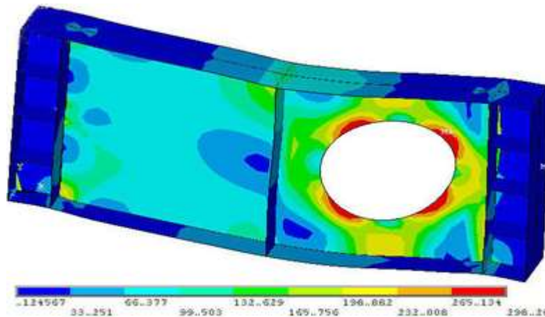
Figure (9): Von Mises stress distribution of plate girder (PGO) at failure
