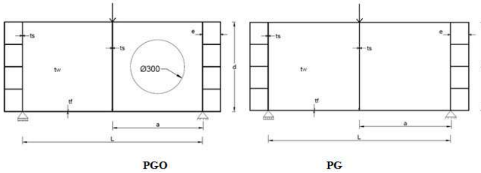
(2):The reference plate girders PG and PGO
