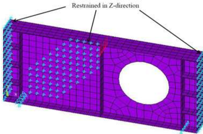
Figure(7): Applied load and Boundary Condition.
