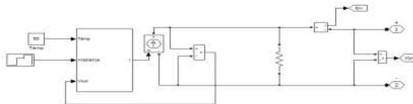
Fig 6 pv subsystem
