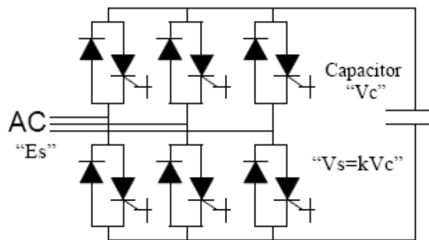
Fig.2 pulses statcom.
