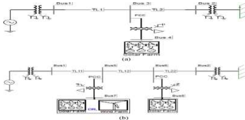
Fig3. Single-line diagram of (a) study system I with a single solar farm (DG) and (b) study system II with a solar farm (DG) and a solar/wind farm (DG).
