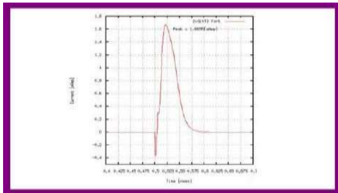
Fig: The peak current behavior of two LVT buffers
