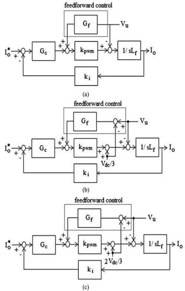
Fig 6. Model of the seven-level inverter under different range of utility voltage, (a) in the range of smaller than V_{dc}/3 , (b) in the range of ( V_{dc}/3 , 2V_{dc}/3 ), (c) in the range of higher than 2V_{dc}/3 .
