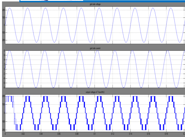
Fig.9. simulation results for the ac side of the seven-level inverter: (a) grid voltage, (b) inverter current (c) output voltage of seven-level inverter.
