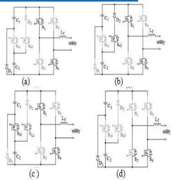
Fig 4 Operation of the seven-level inverter in the positive half cycle, (a) Mode 1, (b) mode 2, (c) mode 3, and (d) mode 4.
