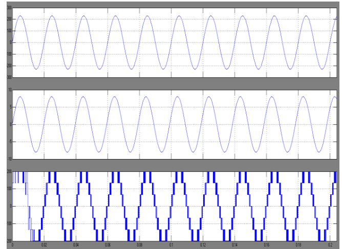
Fig.12. simulation results for the ac side of the seven-level inverter: (a) grid voltage, (b) inverter current (c) output voltage of seven-level inverter.
