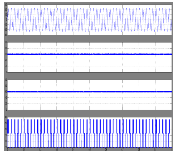
Fig. 13. simulation results for (a) grid voltage, (b) voltage of capacitor C1, (c) voltage of capacitor C2, and (d) output voltage of the capacitor selection circuit.
