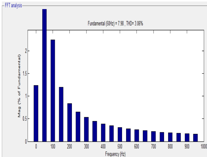
Fig.11. FFT analysis for inverter current.
