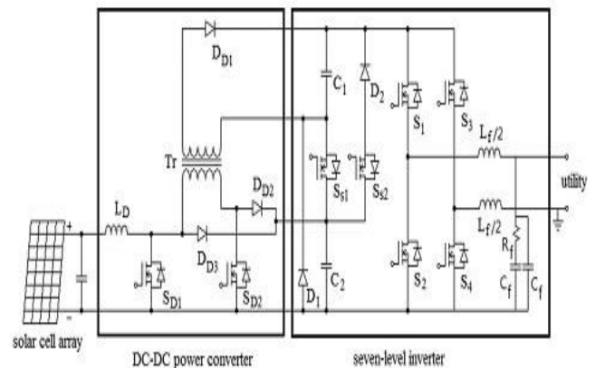
Fig.7. Configuration of the proposed solar power generation system for suppressing the leakage current.
