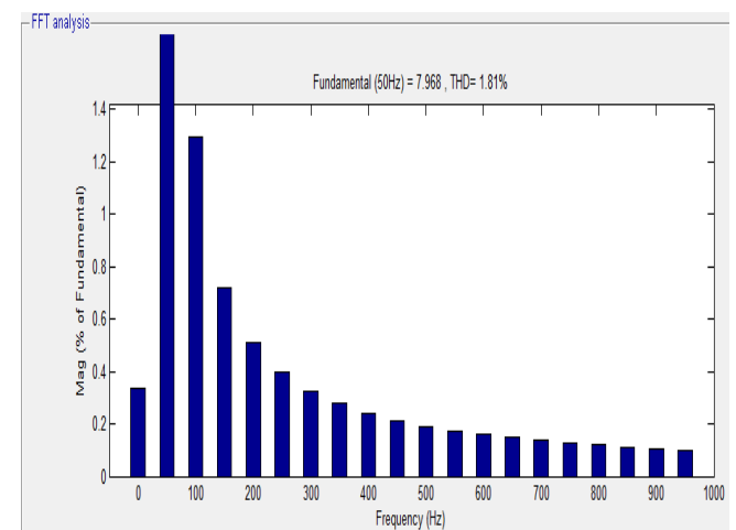
Fig.14. FFT analysis for inverter current.
