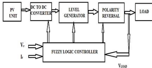
Fig1. Block Diagram of Proposed Solar Power Generation System.
