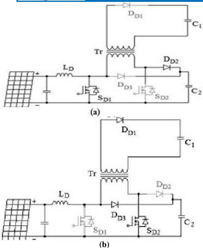
Fig.3. Operation of dc-dc power converter: (a) S_{D1} s on and (b) S_{D1} s off.
