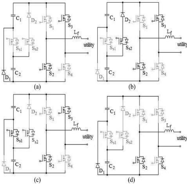
Fig.5. Operation of the seven-level inverter in the negative half cycle: (a) Mode 5, (b) mode 6, (c) mode 7, and (d) mode 8.
