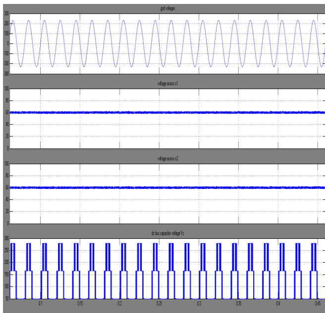
Fig. 10. simulation results for (a) grid voltage, (b) voltage of capacitor C1, (c) voltage of capacitor C2, and (d) output voltage of the capacitor selection circuit.
