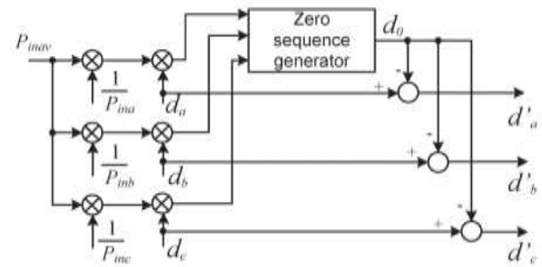
Fig. 6. Modulation compensation scheme.
