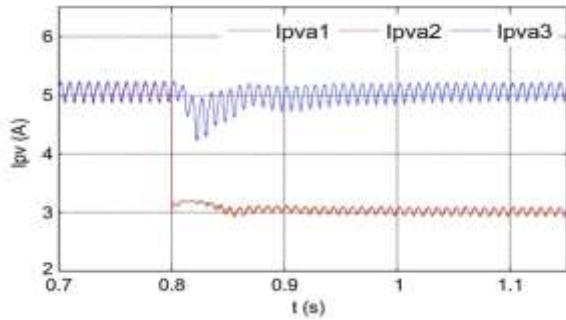
Fig. 9. PV currents of phase a with distributed MPPT ( T = 25^{\circ}C )
