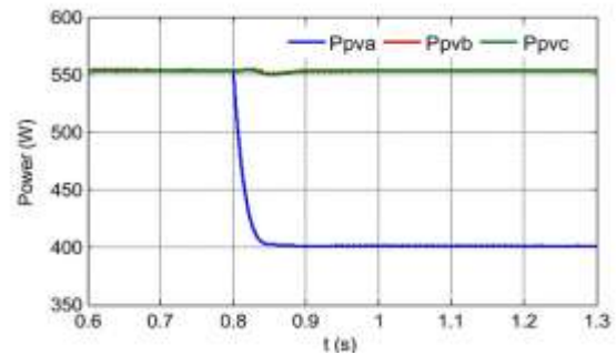
Fig. 11. Power extracted from PV panels with distributed MPPT.
