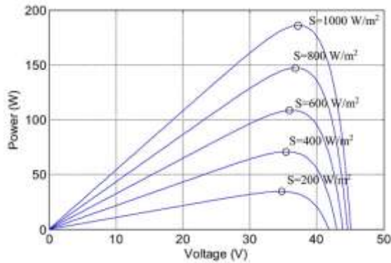
Fig. 4. P - V characteristic under the different irradiance
