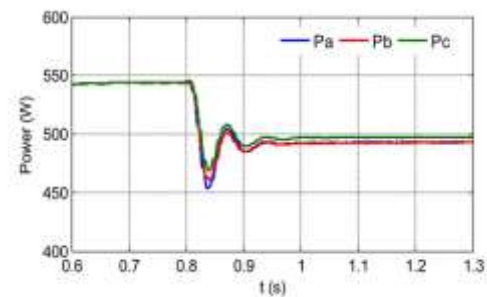
Fig. 12. Power injected to the grid with modulation compensation
