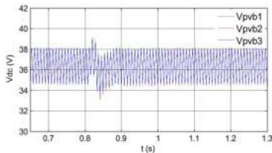
Fig. 10. DC-link voltages of phase b with distributed MPPT ( T = 25^{\circ}C ).
