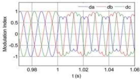
Fig. 7. Modulation indices before and after modulation compensation.
